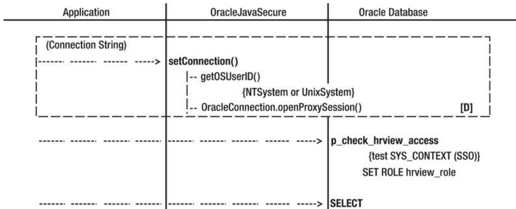
Figure 8-1. SSO procedure
